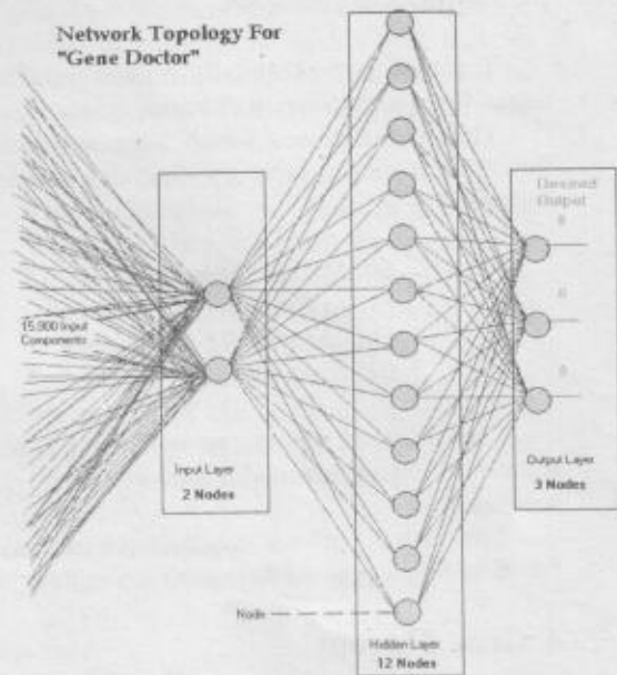
Figure 2 graphically illustrates topology of the Artificial Neural Network used in "Gene Doctor".
